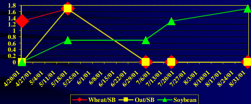
Cover Crop vs White Mold Apothecia counts / meter 2 -Wisconsin
